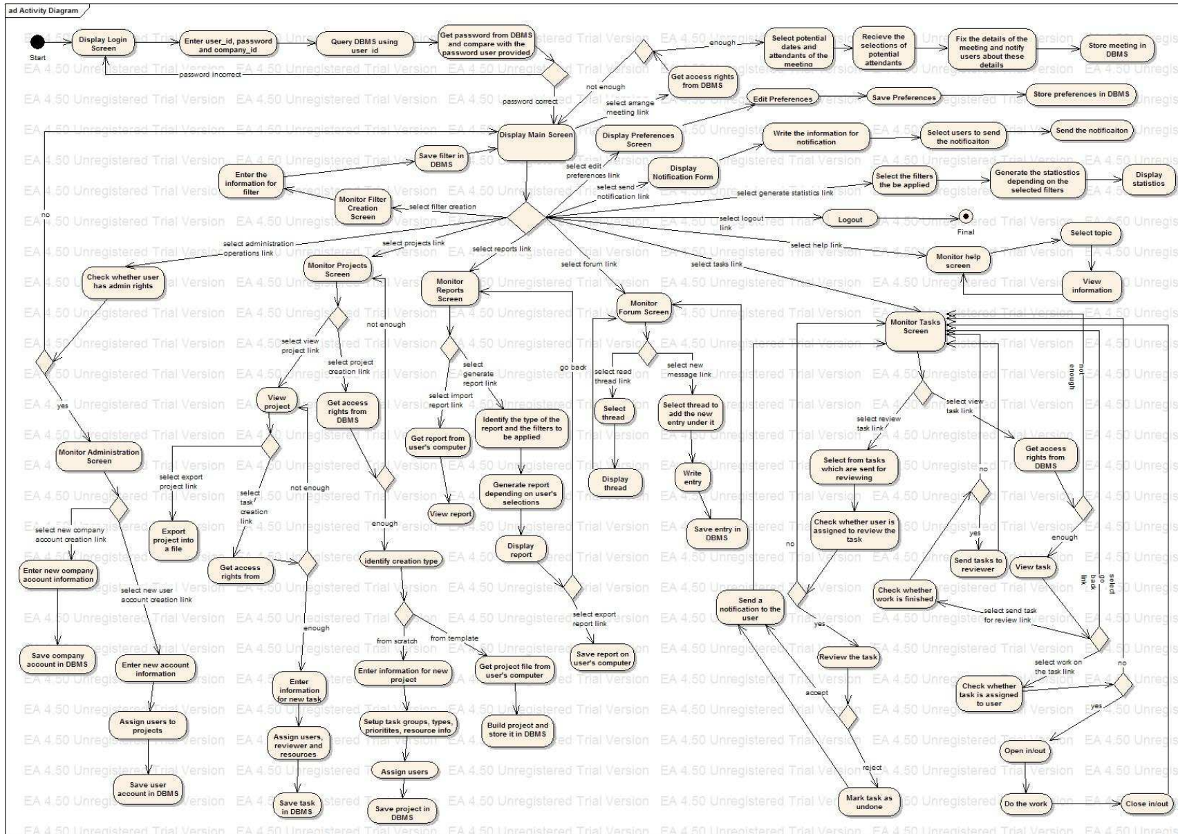
Activity Diagram
