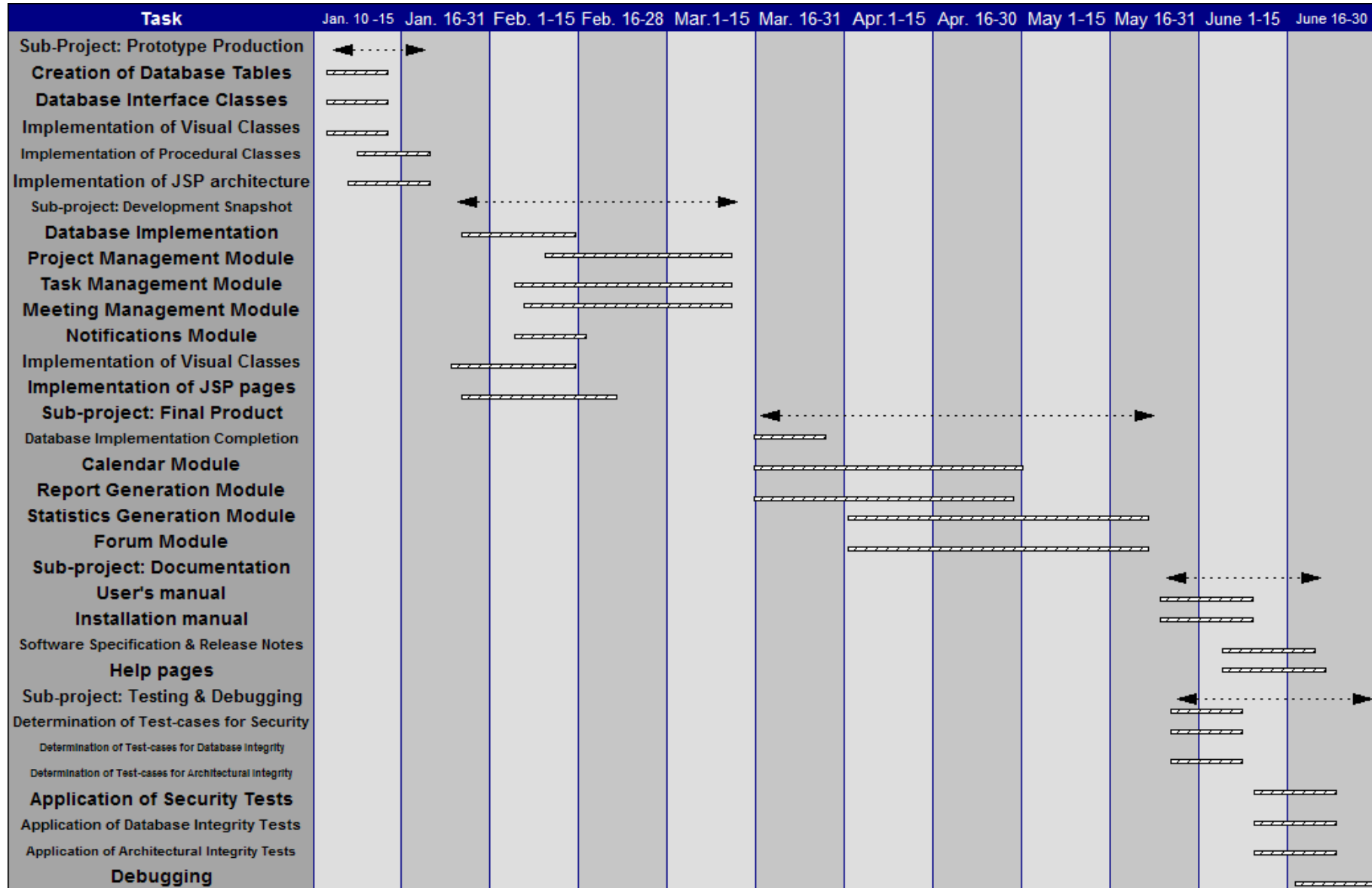
Gantt Chart
