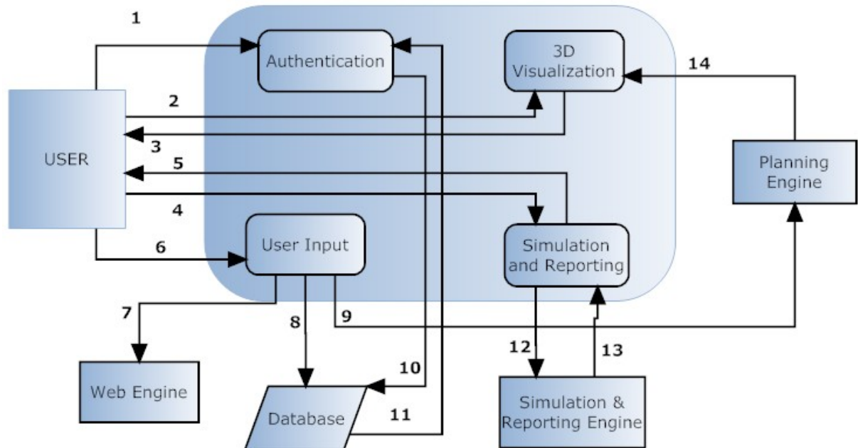
Level2 Data Flow Diagram for User Interaction Engine
