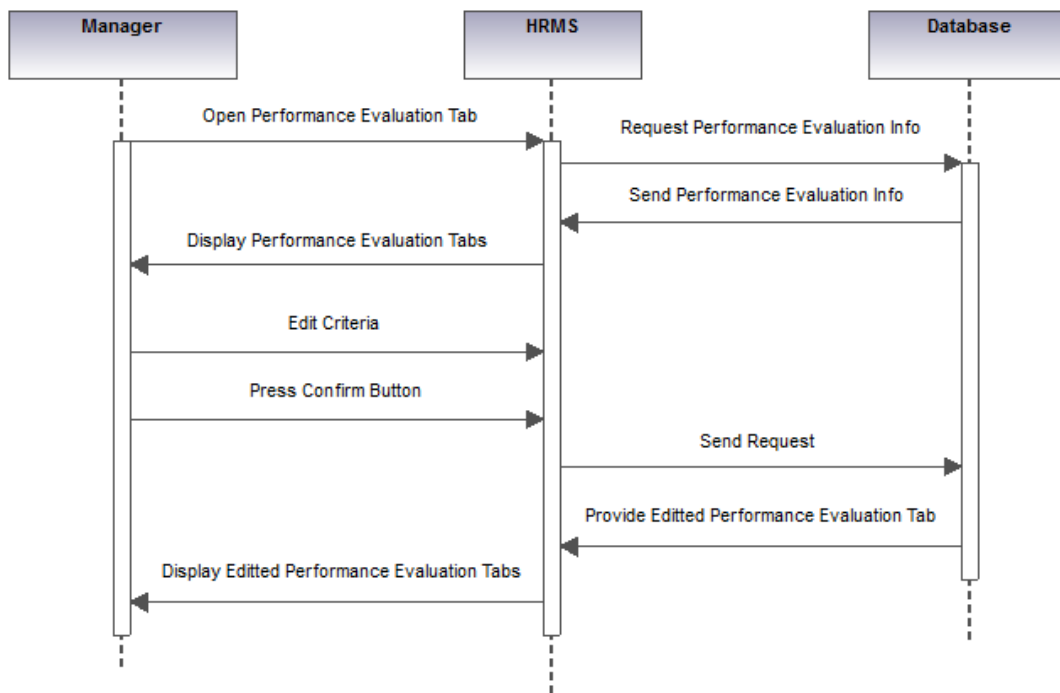
7.2.2.2: Sequence Diagram of manager to edit Performance Evaluation Report
