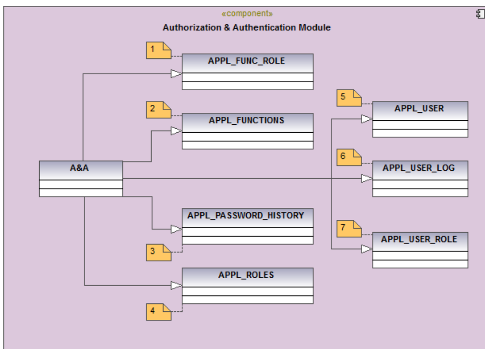
Figure 7.4.2.1 Entity Relation Diagram of Authorization&Authentication Module
