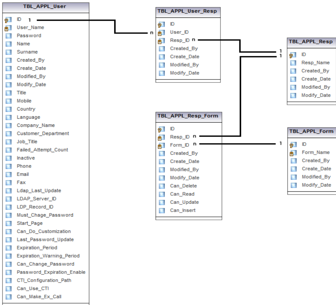
Figure 7.5.1.2: Relation between Database tables of Authentication & Authorization Module
