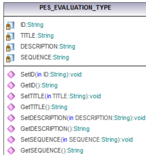
Figure 4.1.1.2.3.1.1: Class Diagram of Evaluation Type Entity
