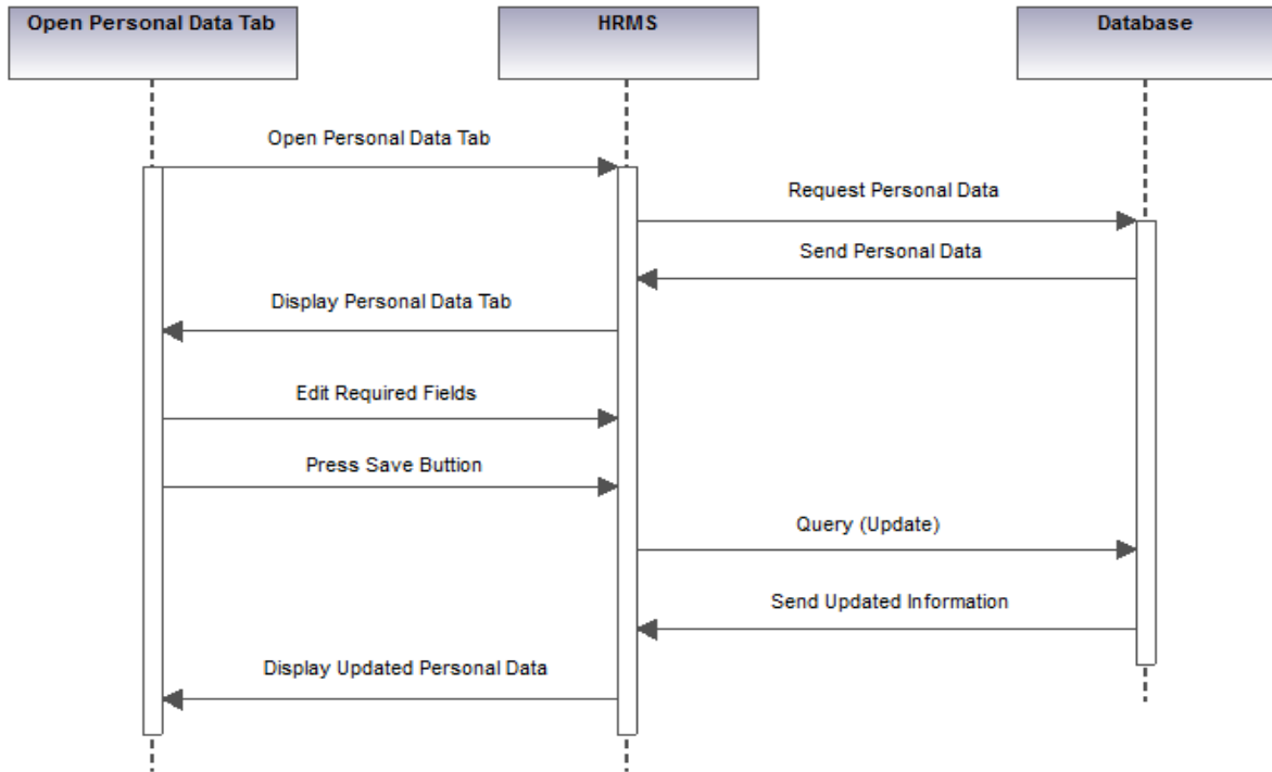
Figure 5.2.2.3.2.1: Sequence Diagram for Personal Data Module
