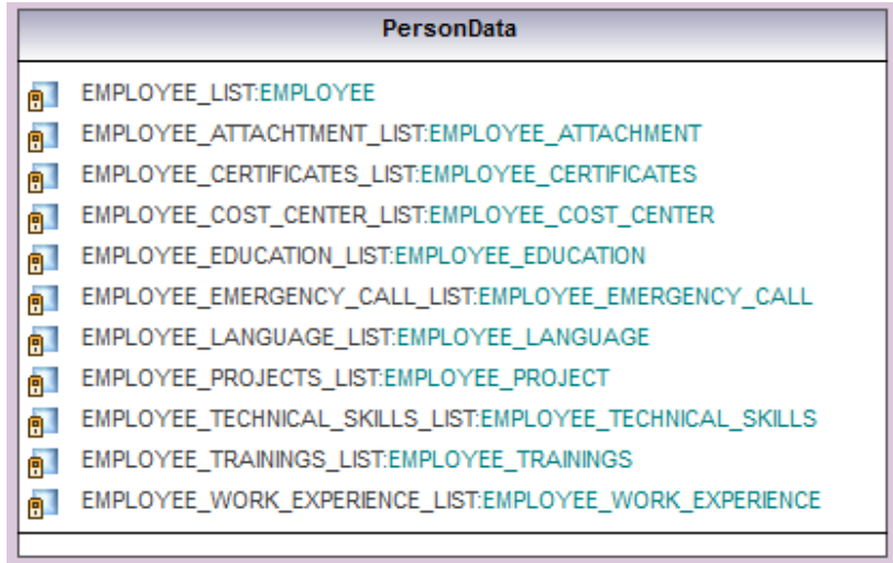
Figure 4.1.1.1.1: Class Diagram of PersonalData
