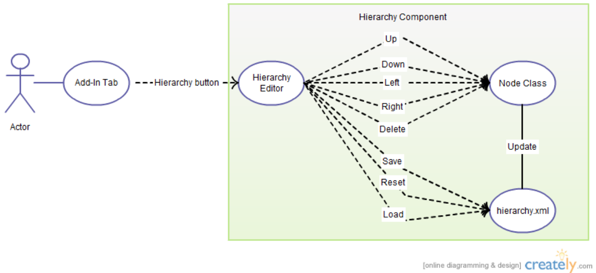
Figure 7.1 : Hierarchy Component Use-Case Diagram
