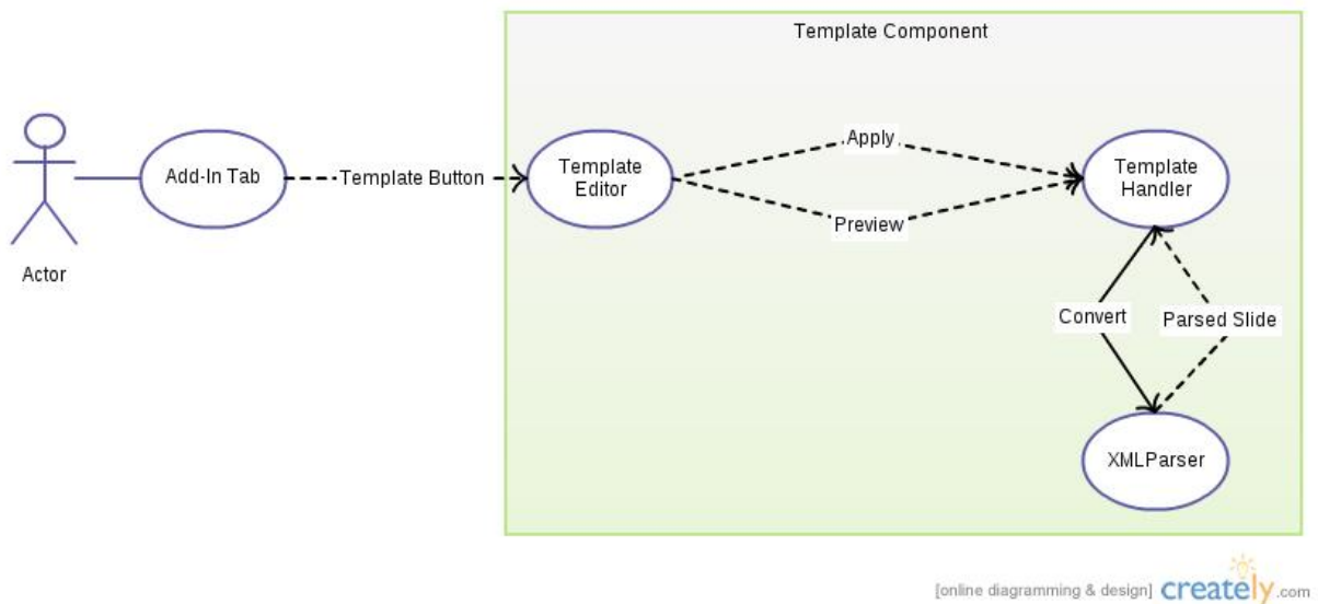
Figure 7.2 : Template Component Use-Case Diagram
