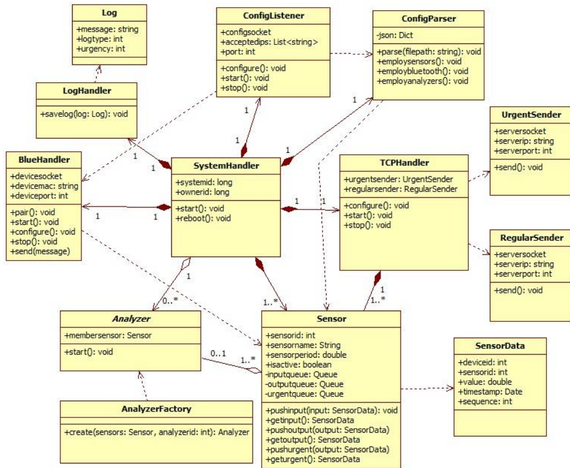
Figure 6 Intermediate Device UML Diagram
