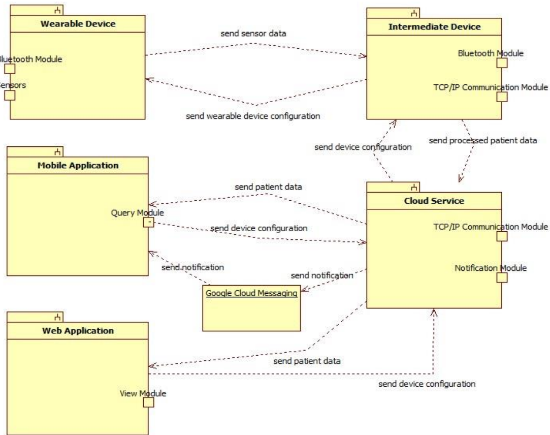
Figure 8 Dependency Diagram
